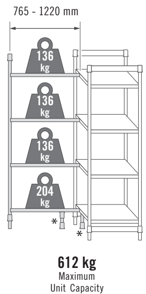
Corner Unit with 2 Dunnage Stands
