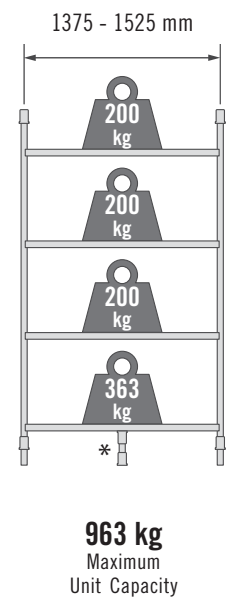
Single Unit with Dunnage Stand
